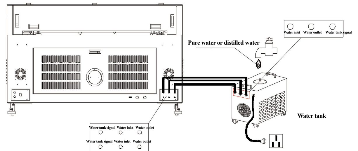
Fig. 4-2 Connection of Water Tank
