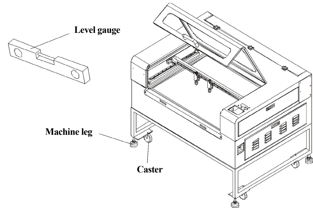
Fig. 4-1 Leveling
