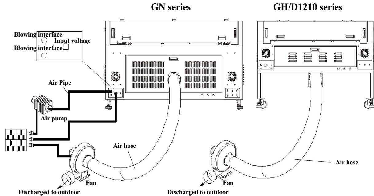
Fig. 4-3 Connection of Fan/Power Cord
