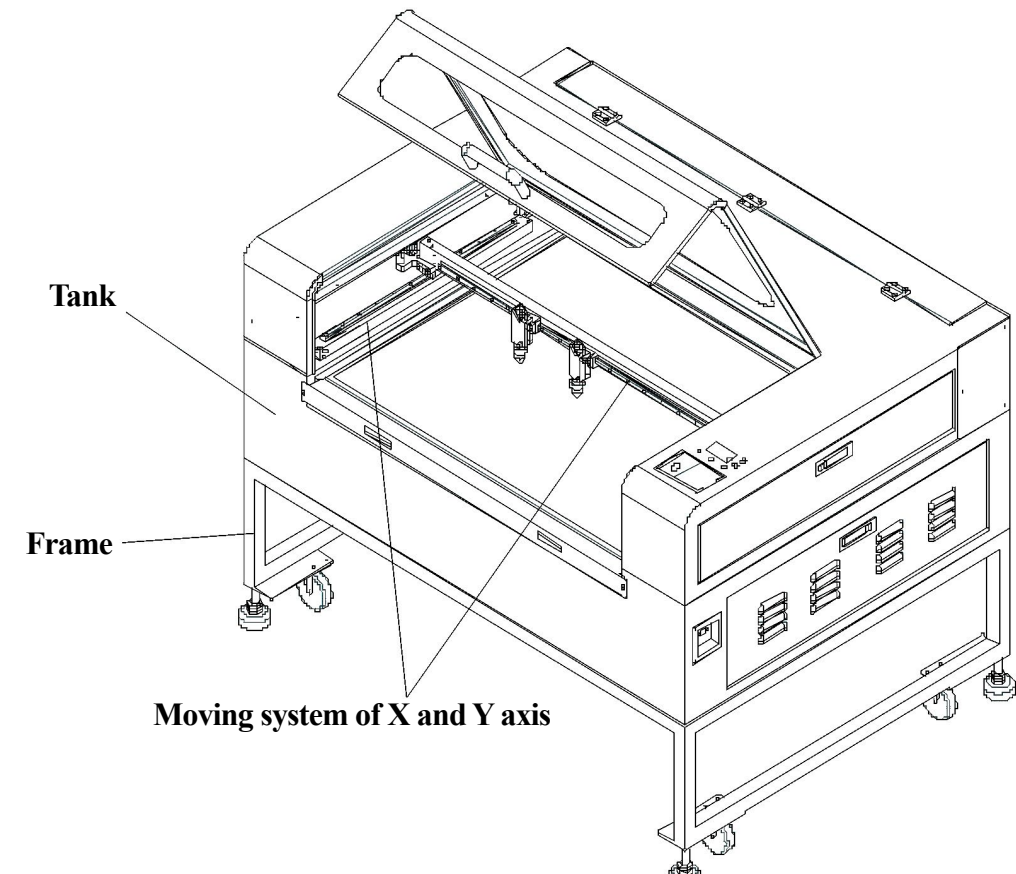
Fig. 3-4 GH /D1210 Series
